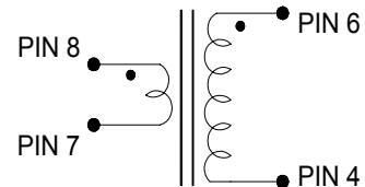
Schematic
